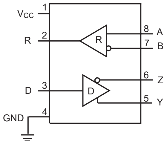
TK490 Pinout (Top View)
