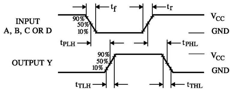
Figure 1. Switching Waveforms
