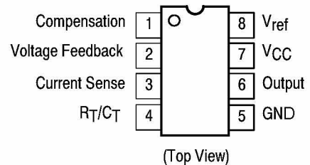
PIN CONNECTIONS
