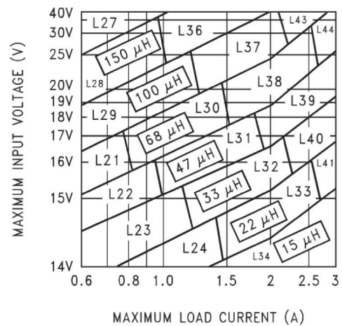
TK2596-12
