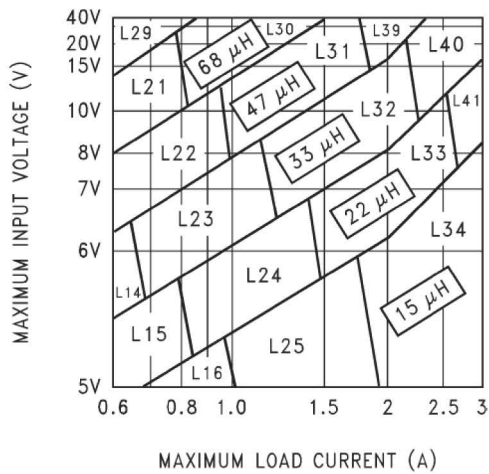
TK2596-3.3
