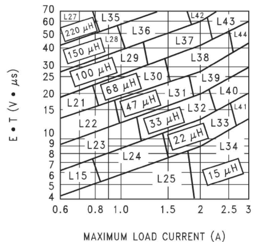
TK2596-ADJ
