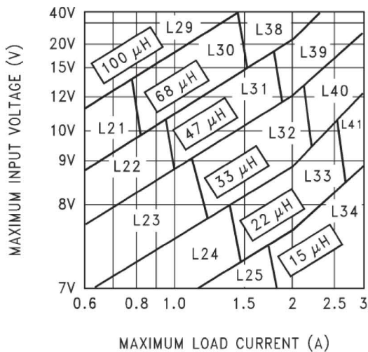
TK2596-5.0
