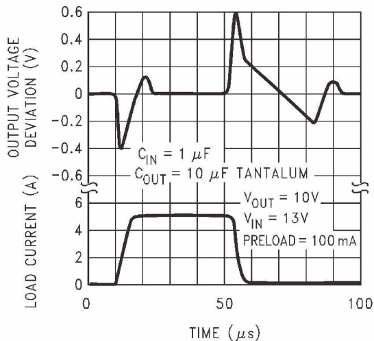
Figure 8. LM1084-ADJ Load Transient Response
