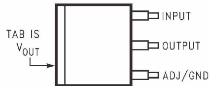
3-Pin TO-263 Package Top View
