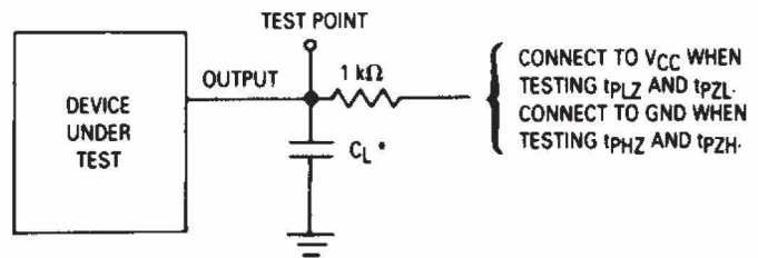
Figure 6. Test Circuit
