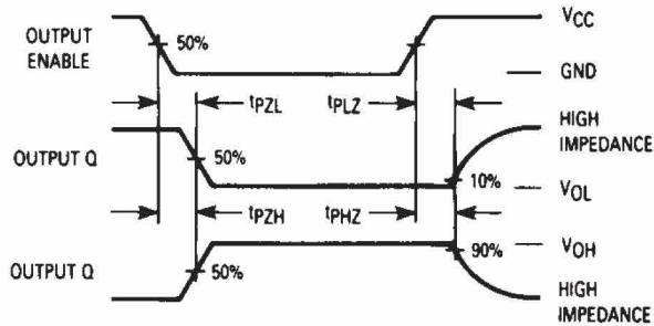
Figure 3. Switching Waveforms
