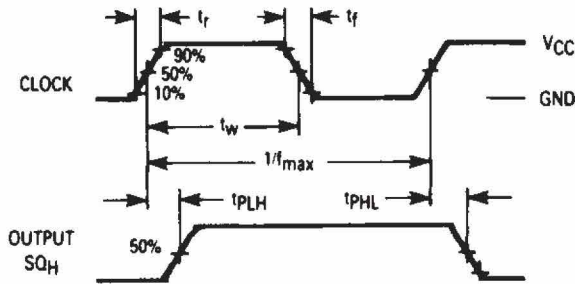
Figure 1. Switching Waveforms
