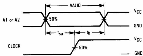
Figure 3. Switching Waveforms
