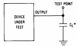
Figure 4. Test Circuit
